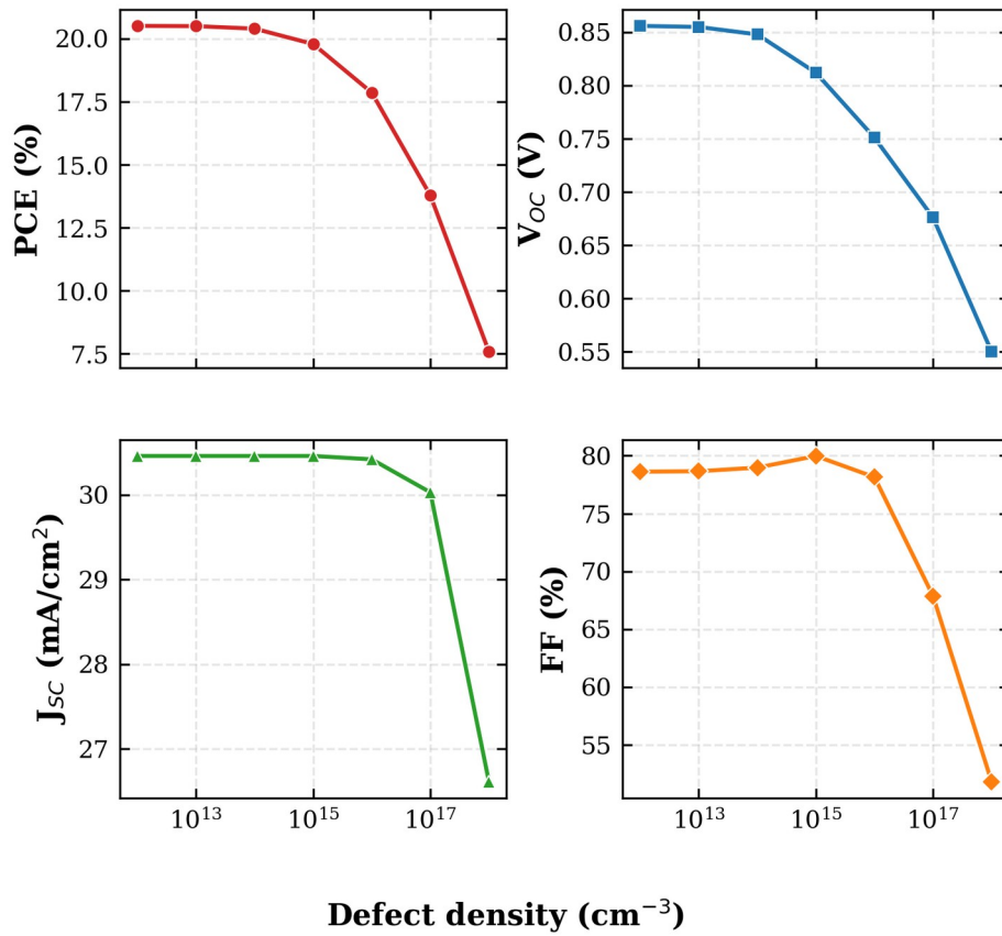
FIG. 4. Variation of PCE, V OC , J SC , and FF with RbGeI 3 absorber defect density. The device is essentially insensitive to defect densities below 10 15 cm -3 but degrades sharply at higher values due to SRH recombination.
