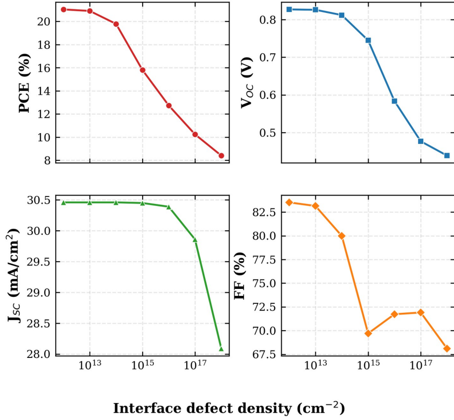
FIG. 7. Variation of PCE, V_{OC} , J_{SC} , and FF with the \text{TiO}_2/\text{RbGeI}_3 interfacial defect density. Performance degrades sharply above 10^{14} \text{ cm}^{-2} , indicating high sensitivity to absorber/ETL interface quality.
